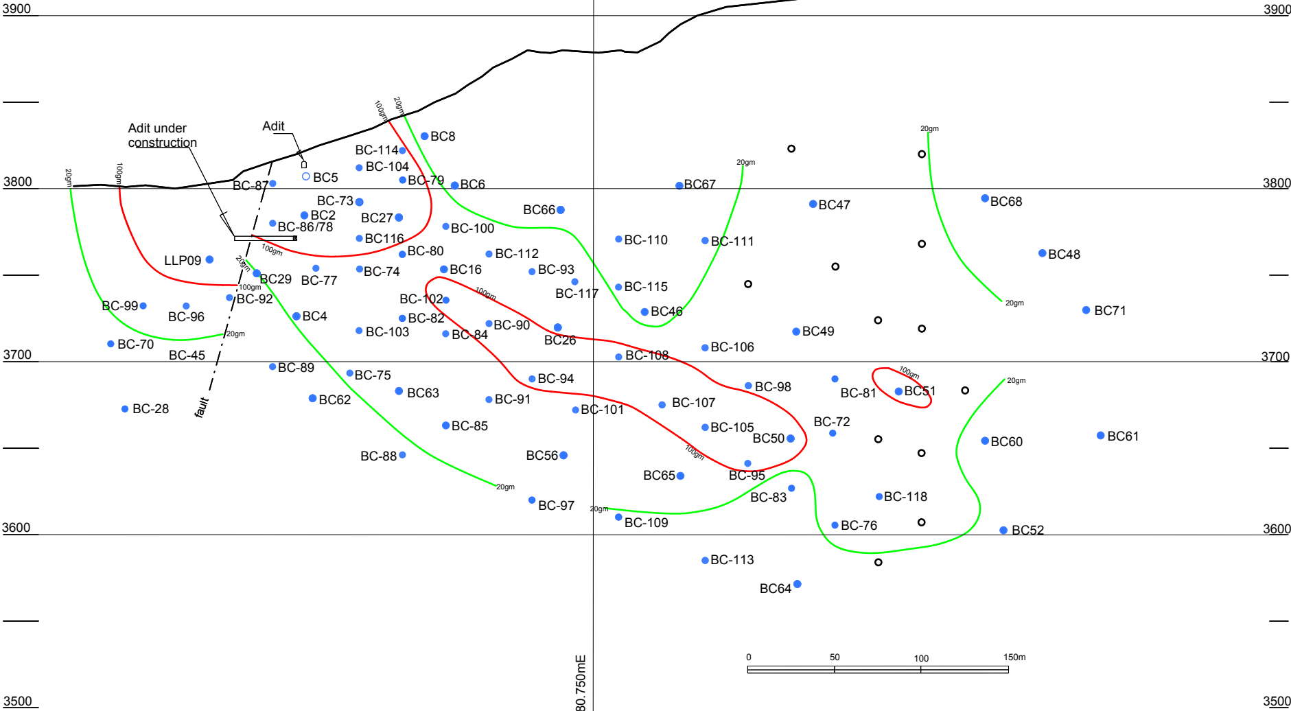
ALEJANDRA VEIN - LONG SECTION VIEW Showing 20 g.m and 100 g.m gold contours
