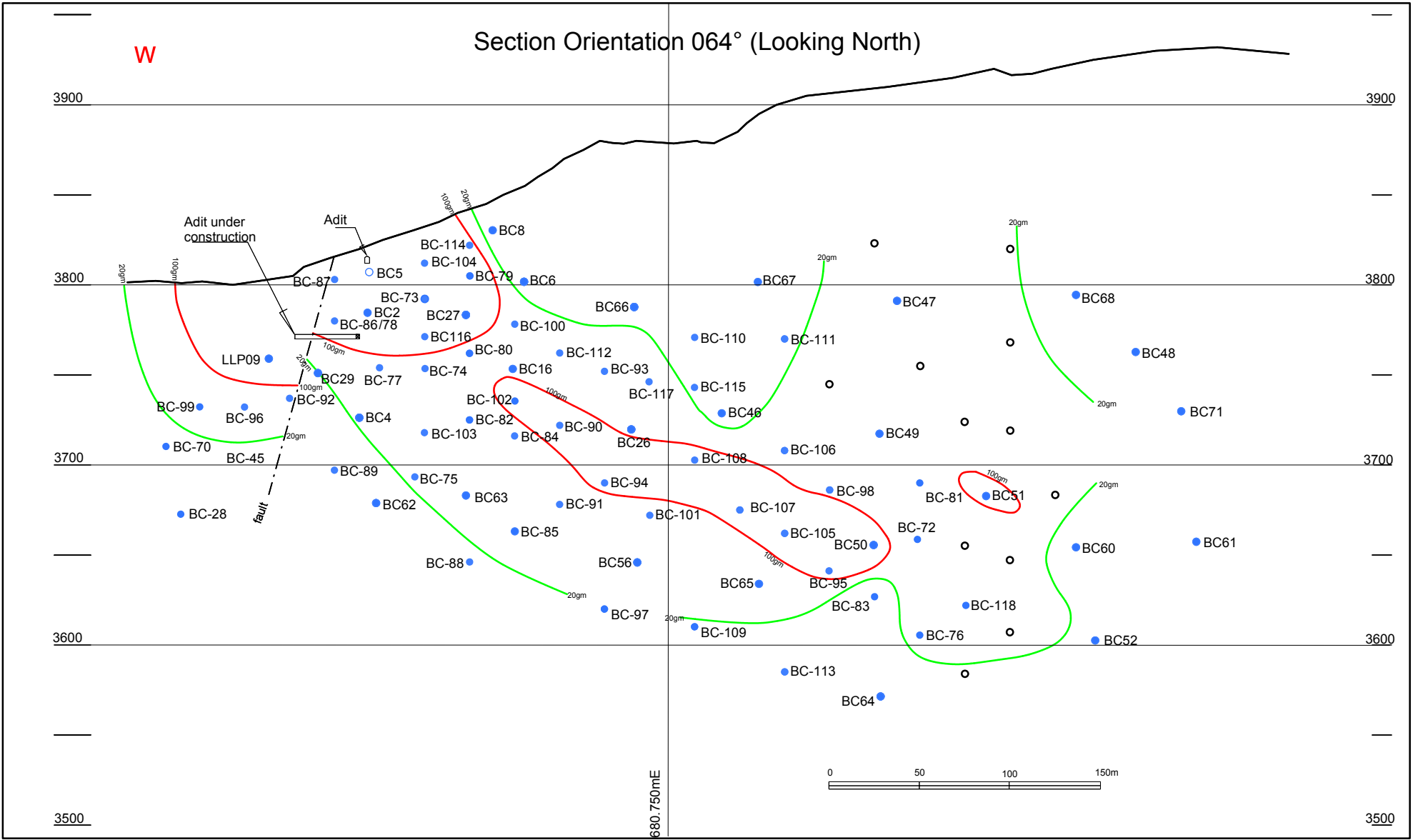
ALEJANDRA VEIN - LONG SECTION VIEW Showing 20 g.m and 100 g.m gold contours
